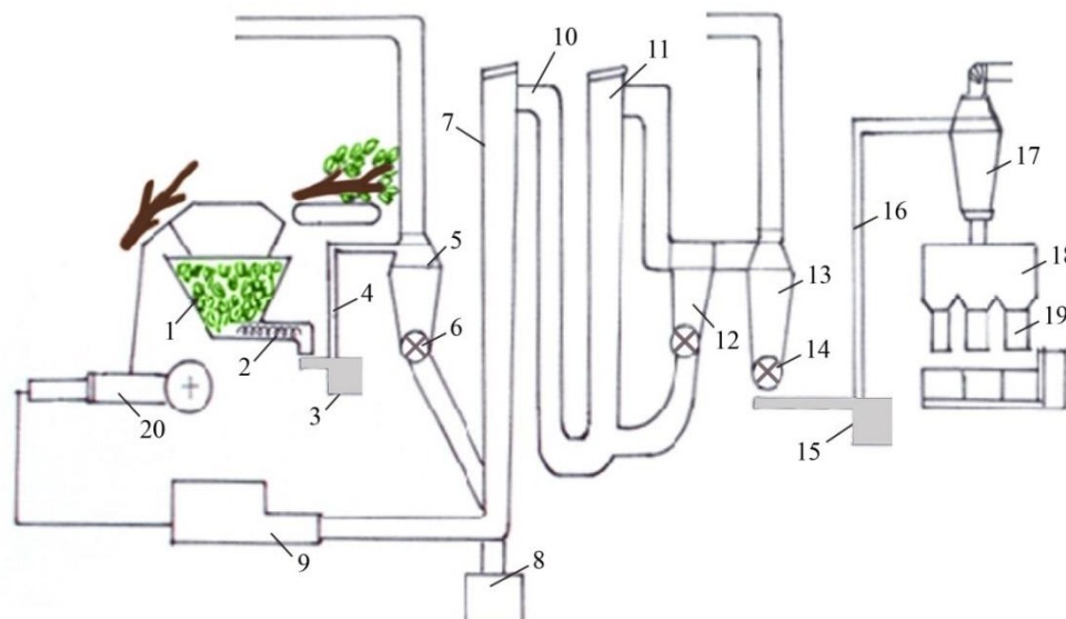
Figure 7: Technological scheme for the production of vitamin-mineral flour: 1. Bunker for receiving WG, 2.Screw conveyor, 3. Crusher, 4. Pneumatic conveyor, 5. Bunker for receiving rough chips, 6. Dosing unit, 7. First drying column, 8. Bunker for receiving waste material from the first drying column (wood and bark particles), 9. Furnance, 10. Second drying column, 11. Third drying column, 12. Separator of residual wet material, 13. Cyclone, 14. Dosing unit, 15. Mill, 16. Pneumatic conveyor, 17. Cyclone, 18. Bunker of VMF, 19. Line for filling and sewing bags with VMF (according to Tomčuk et Tomčuk, 1966)
