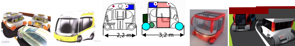
FIG. 5 - Several design pictures of a coupemobile. With the axles retracted, the length of the vehicle is only 2.2 m, while the wheelbase is increased by 1 m while driving. It is possible to enter the trains laterally and to park perpendicular to the pavement.
