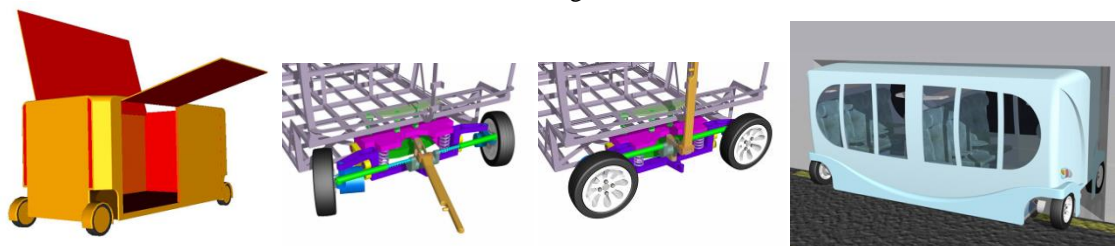
FIG.4 - The freight and passenger transport modules are equipped with its own low power electric drive for independent local manipulation. The wheels can be swiveled 90^\circ for lateral loading into the railcoach.
